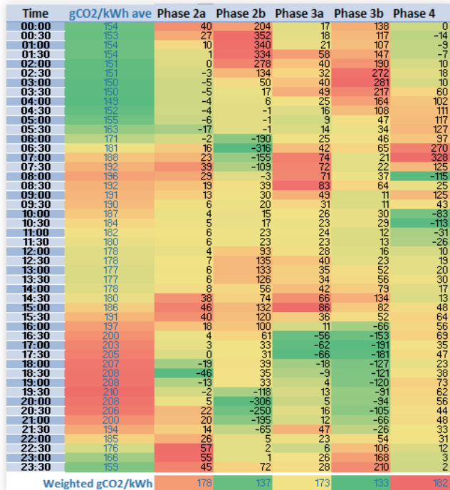
Figure 18: kWh charged by phase and time of day in comparison to average grid carbon intensity
