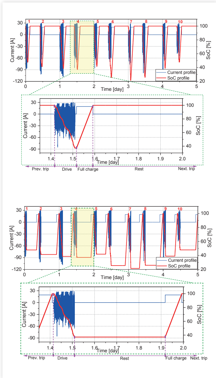
Figure 39: Example STD CHA (top and TS CHA (bottom)
