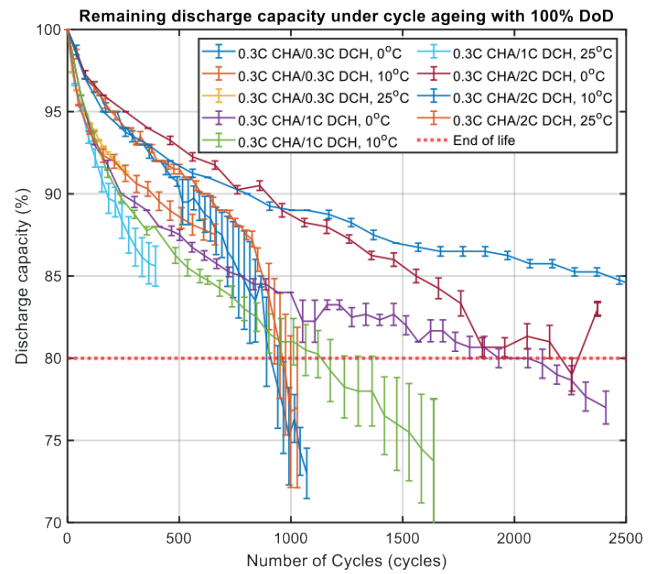
Figure 37: Remaining discharge capacity under cycle ageing with 100% DoD
