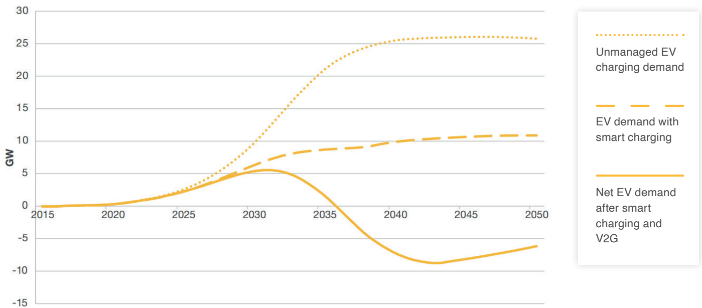
Figure 1: Electric Vehicle charging behaviour at winter peak demand.
