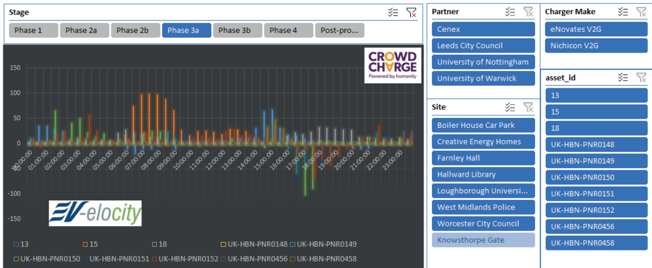
Figure 16: Example charger behaviour in Phase 3a
