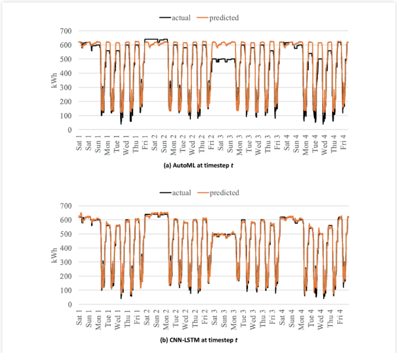
Figure 33: Actual vs predicted capacity for a sample 4-week period. AutoML regressor (a); CNN-LSTM model (b)
