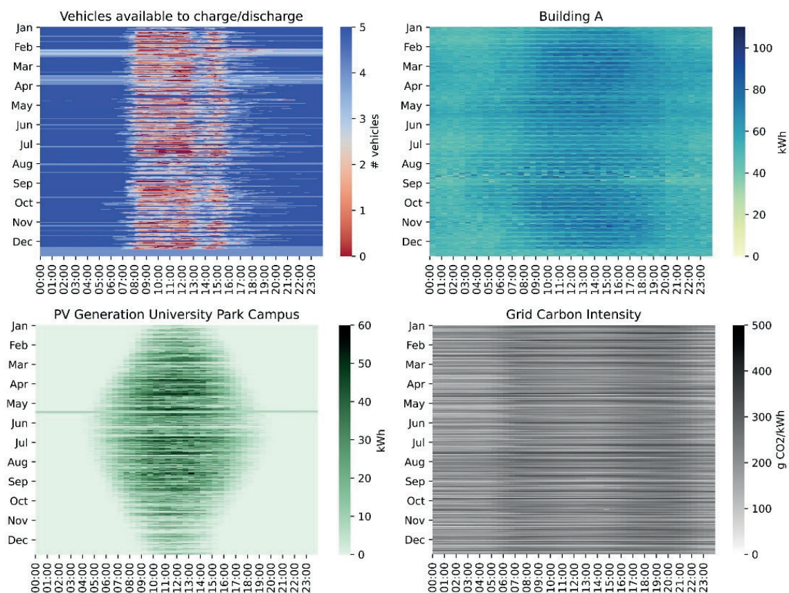
Figure 29: Clockwise from top-left: Fleet availability to charge; electricity demand of Building A; grid CO 2 intensity; and campus solar generation
