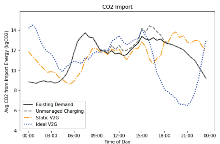
Figure 31: Average daily CO 2 import over one year under three V2G scenarios
