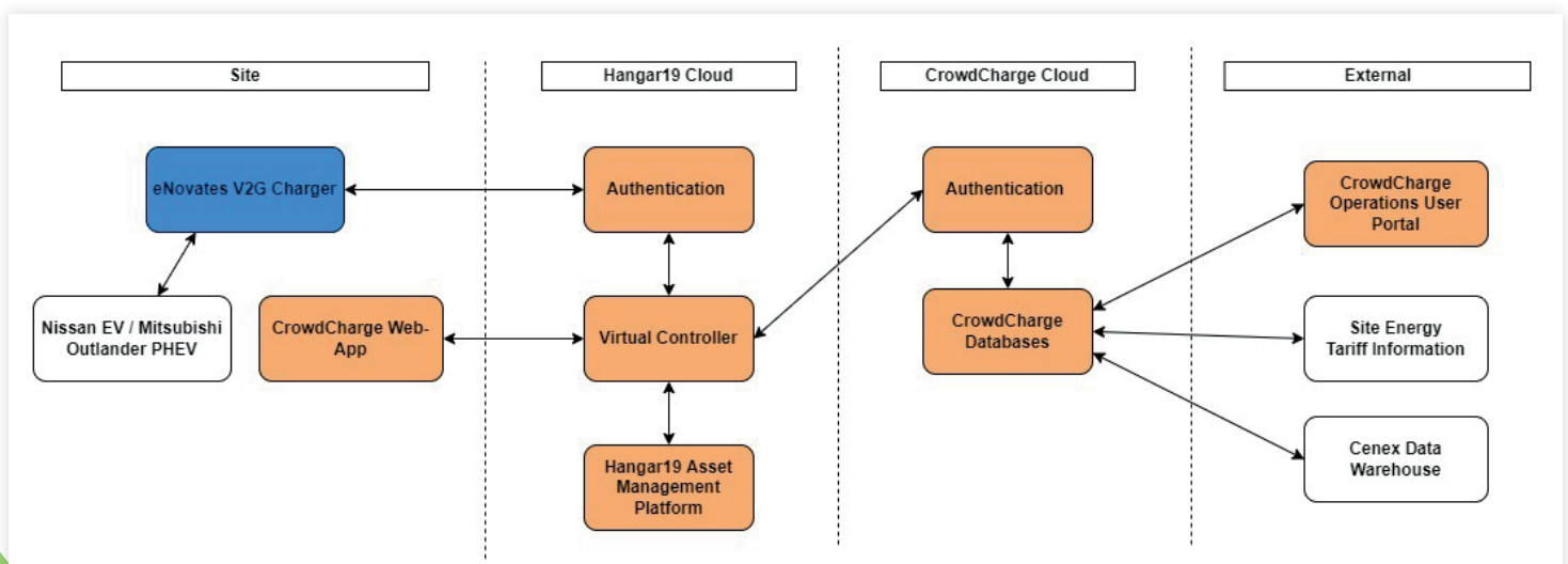
Figure 8: CrowdCharge architecture for eNovates charger
