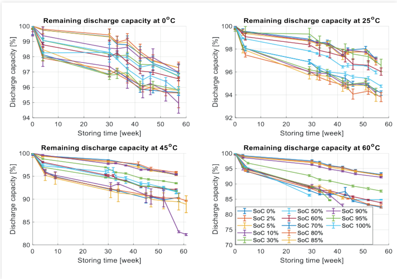
Figure 36: Remaining discharge capacity under calendar ageing for different storage temperatures
